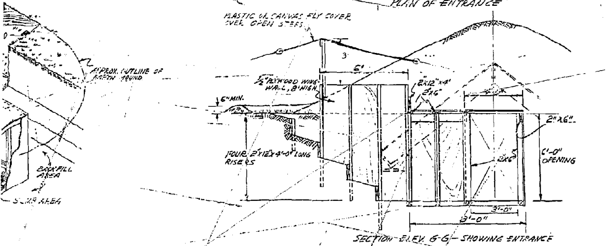
3. A-10.1. "A"-Frame Expedient Shelter, Plans and Elevation.
